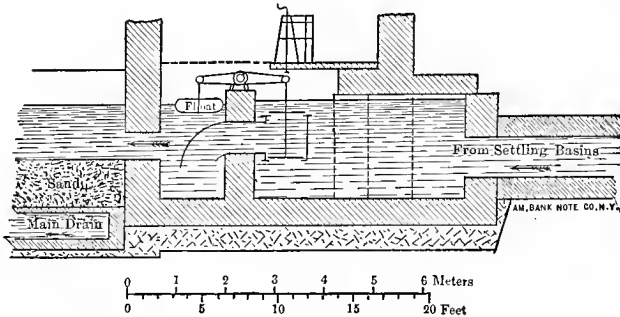
FIG. 11.—REGULATION OF INFLOW USED AT HAMBURG.
